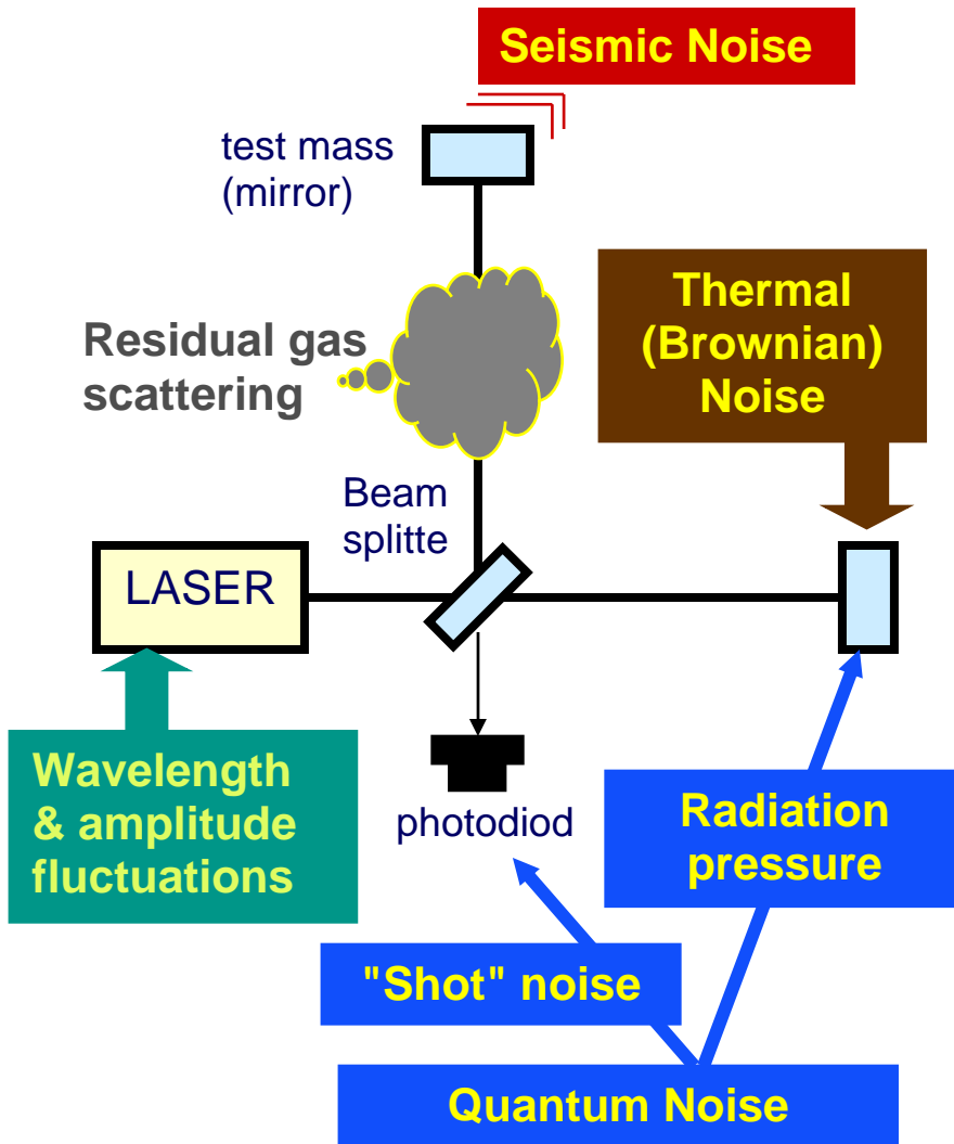
Figure XX – placeholder for new graphics. Noise sources in LIGO.
